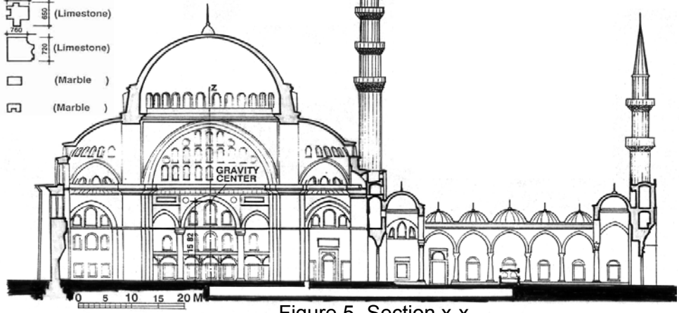
Figure 5 -Section x-x
