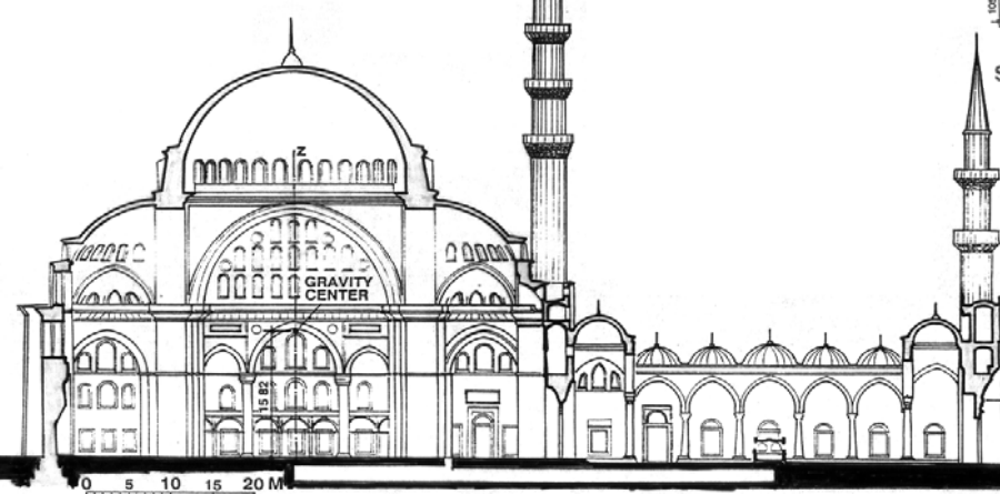
Figure 6 -Section y-y
